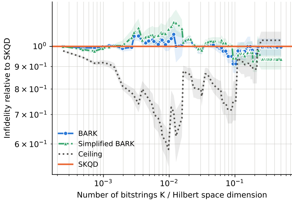
runs per point -- BARK: 6-36, Ceiling: 6-36, SKQD: 6-36, Simplified BARK: 6-36
