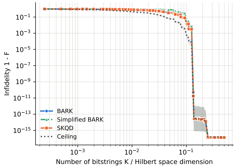
runs per point -- BARK: 8-13, Ceiling: 8-13, SKQD: 8-13, Simplified BARK: 8-13
