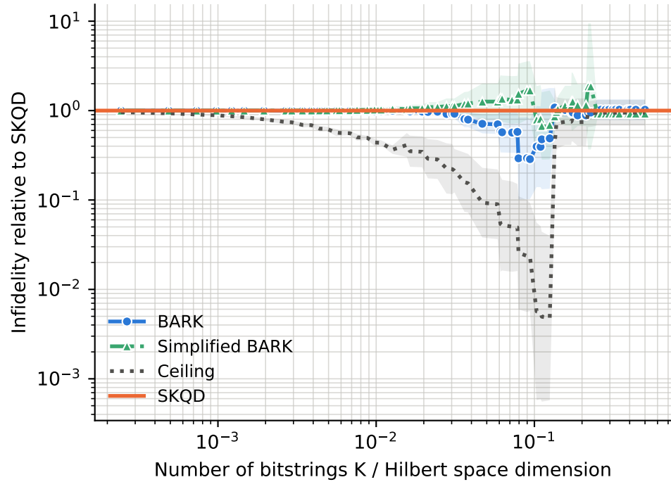
runs per point -- BARK: 8-11, Ceiling: 8-11, SKQD: 8-11, Simplified BARK: 8-11
