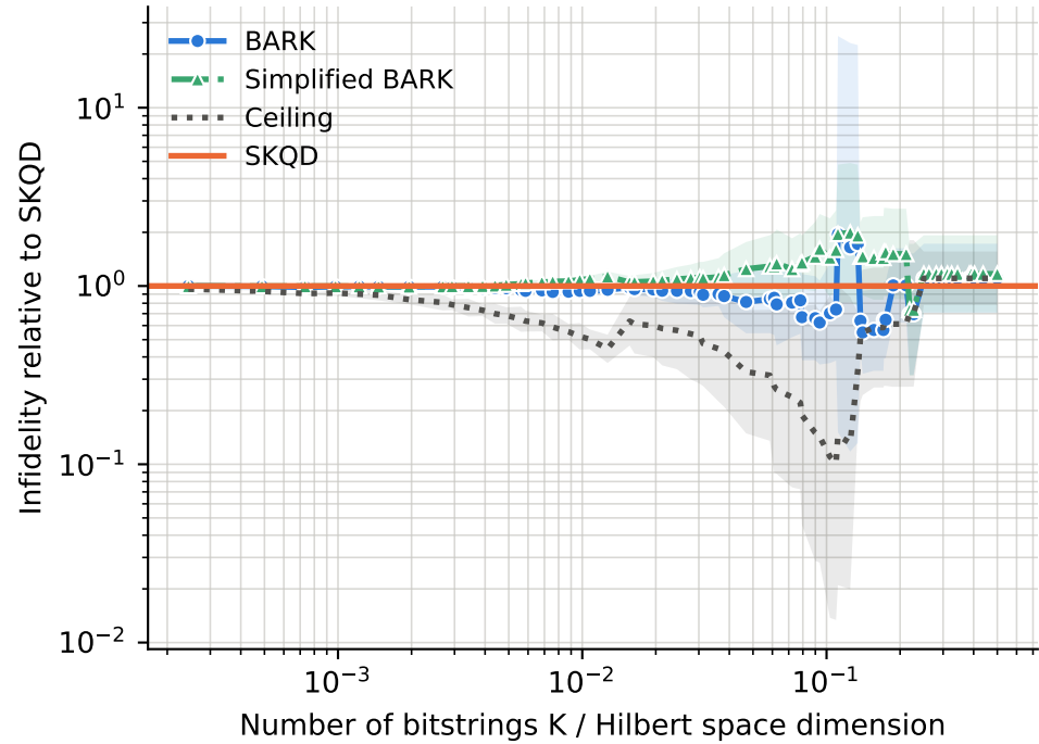
runs per point -- BARK: 2-12, Ceiling: 2-12, SKQD: 2-12, Simplified BARK: 2-12
