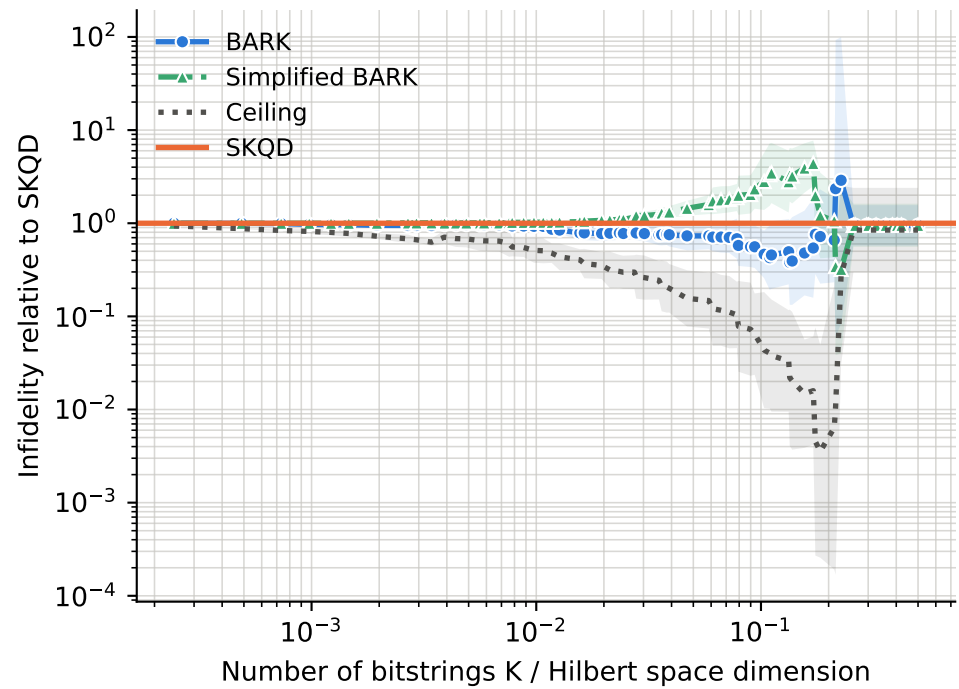
runs per point -- BARK: 4-9, Ceiling: 4-9, SKQD: 4-9, Simplified BARK: 4-9
