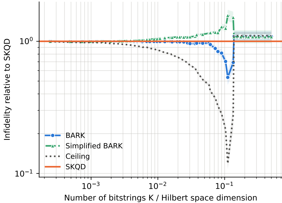
runs per point -- BARK: 12-26, Ceiling: 12-26, SKQD: 12-26, Simplified BARK: 12-26
