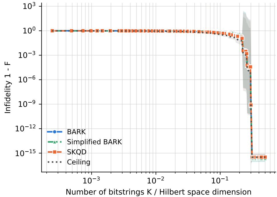
runs per point -- BARK: 2-20, Ceiling: 2-20, SKQD: 2-20, Simplified BARK: 2-20
