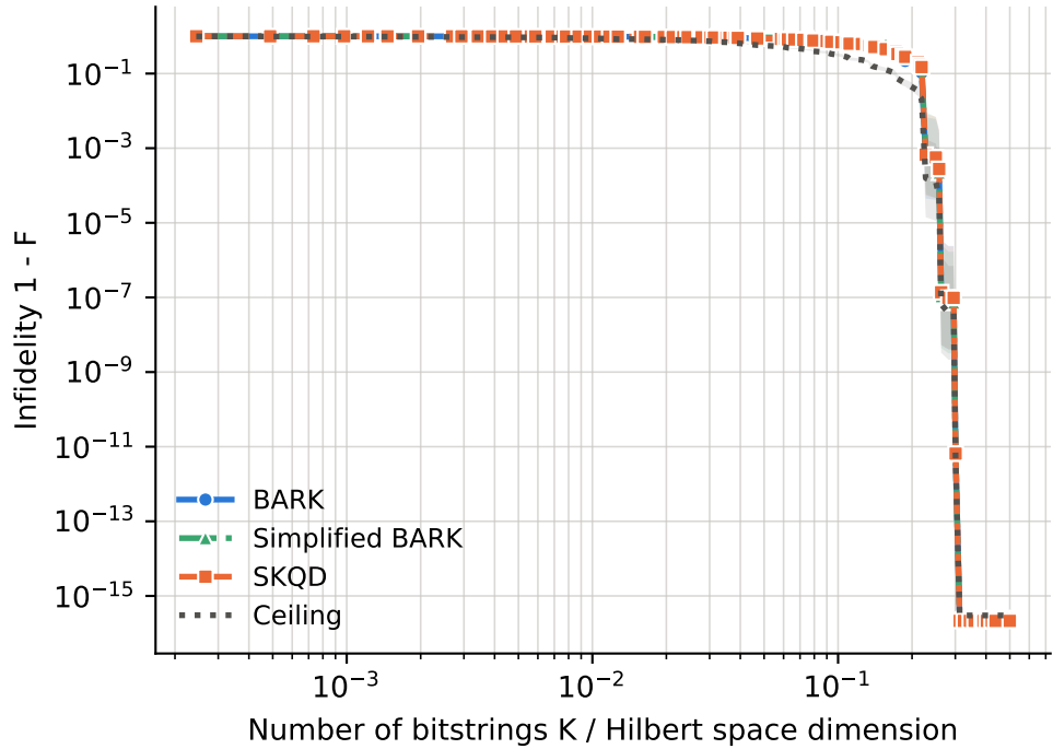
runs per point -- BARK: 4-26, Ceiling: 4-26, SKQD: 4-26, Simplified BARK: 4-26
