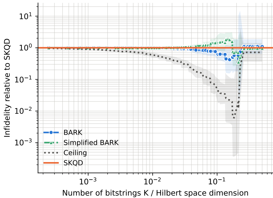
runs per point -- BARK: 9-16, Ceiling: 9-16, SKQD: 9-16, Simplified BARK: 9-16
