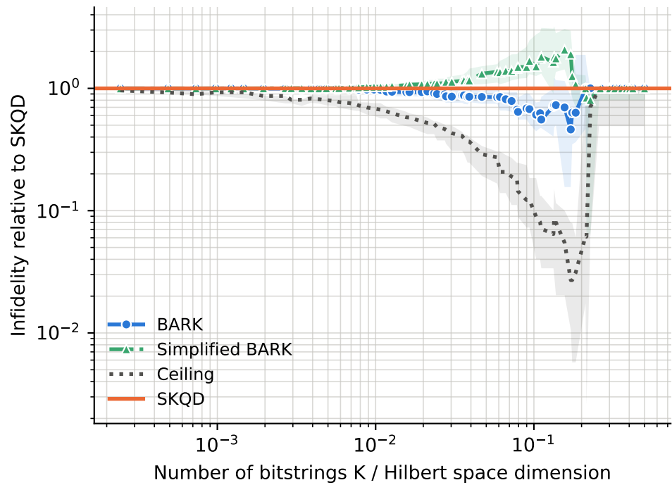
runs per point -- BARK: 8-20, Ceiling: 8-20, SKQD: 8-20, Simplified BARK: 8-20
