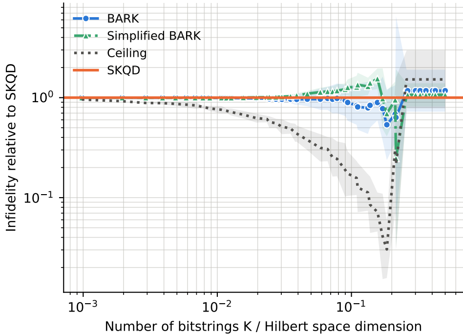
runs per point -- BARK: 6-10, Ceiling: 6-10, SKQD: 6-10, Simplified BARK: 6-10
