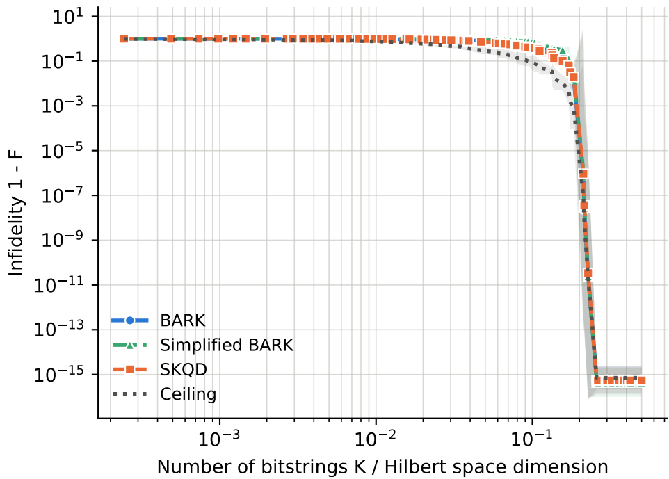
runs per point -- BARK: 2-9, Ceiling: 2-9, SKQD: 2-9, Simplified BARK: 2-9
