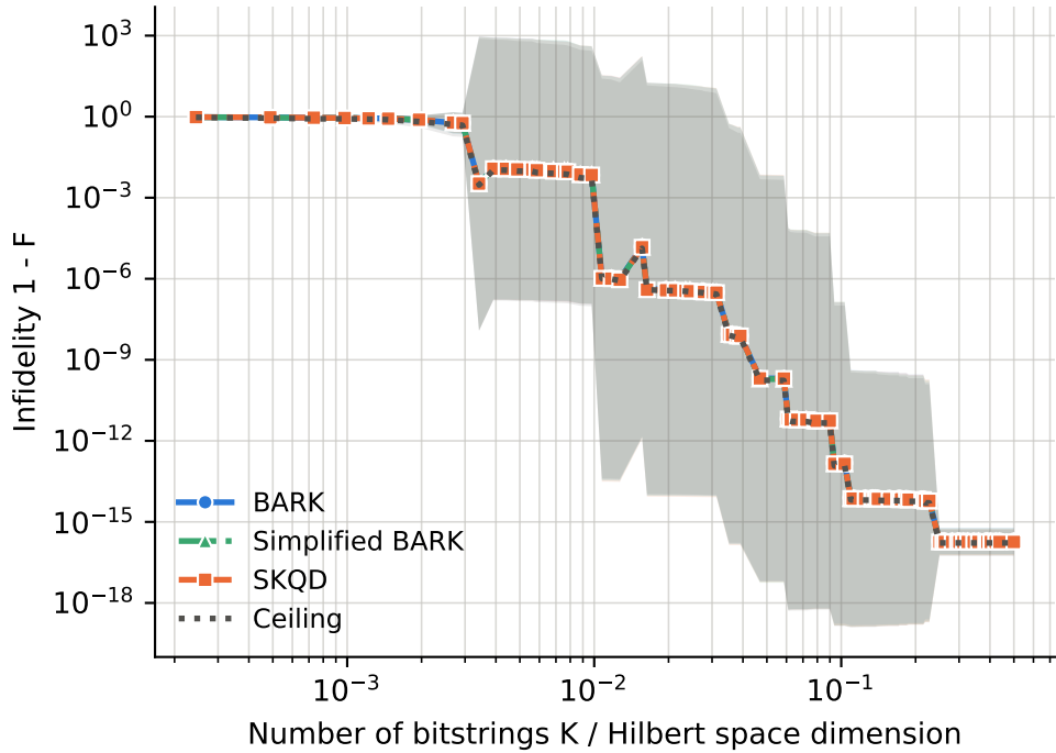
runs per point -- BARK: 18-59, Ceiling: 18-59, SKQD: 18-59, Simplified BARK: 18-59
