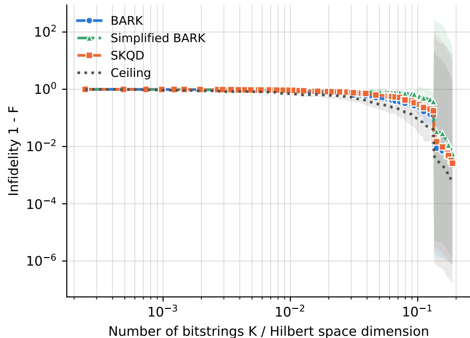
runs per point -- BARK: 1-14, Ceiling: 1-14, SKQD: 1-14, Simplified BARK: 1-14
