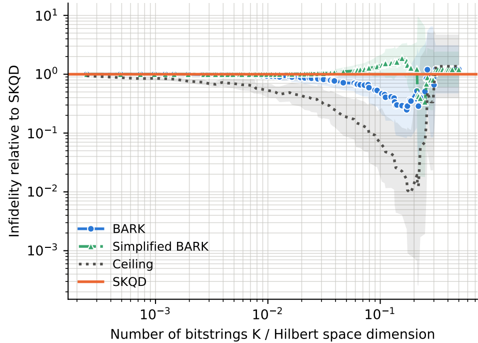
runs per point -- BARK: 6-27, Ceiling: 6-27, SKQD: 6-27, Simplified BARK: 6-27
