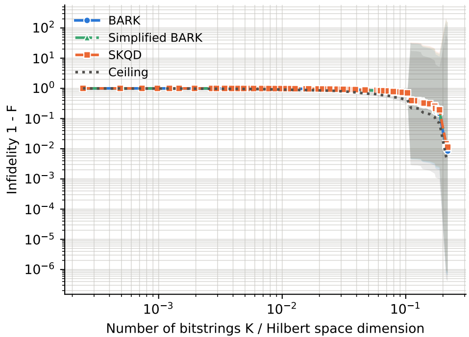
runs per point -- BARK: 17-68, Ceiling: 17-68, SKQD: 17-68, Simplified BARK: 17-68
