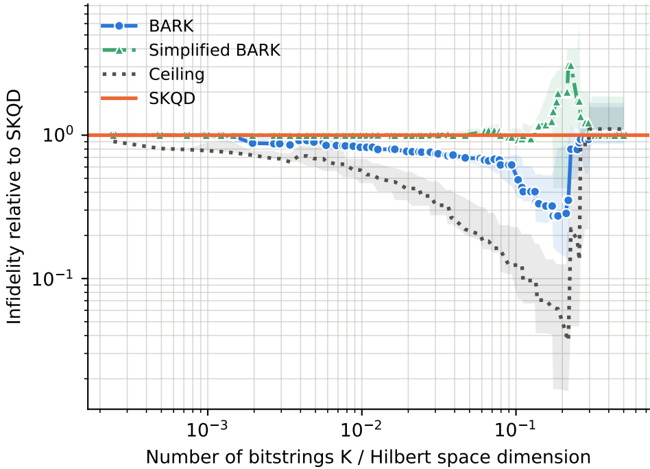
runs per point -- BARK: 6-19, Ceiling: 6-19, SKQD: 6-19, Simplified BARK: 6-19
