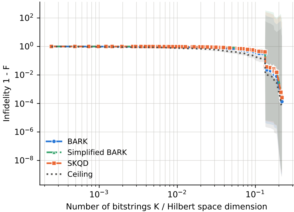
runs per point -- BARK: 11-32, Ceiling: 11-32, SKQD: 11-32, Simplified BARK: 11-32
