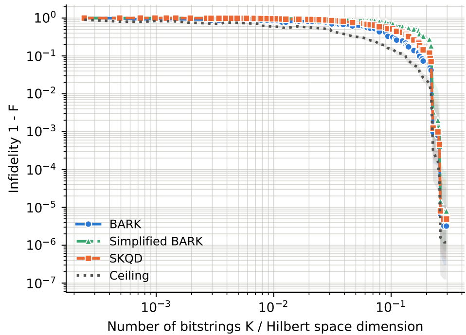
runs per point -- BARK: 4-31, Ceiling: 4-31, SKQD: 4-31, Simplified BARK: 4-31
