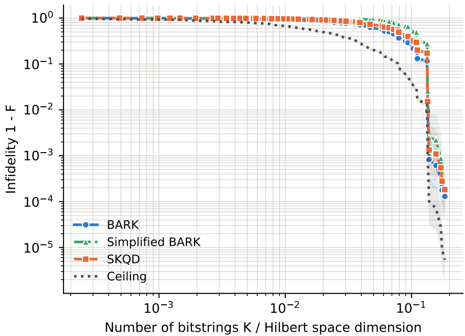
runs per point -- BARK: 24-84, Ceiling: 24-84, SKQD: 24-84, Simplified BARK: 24-84
