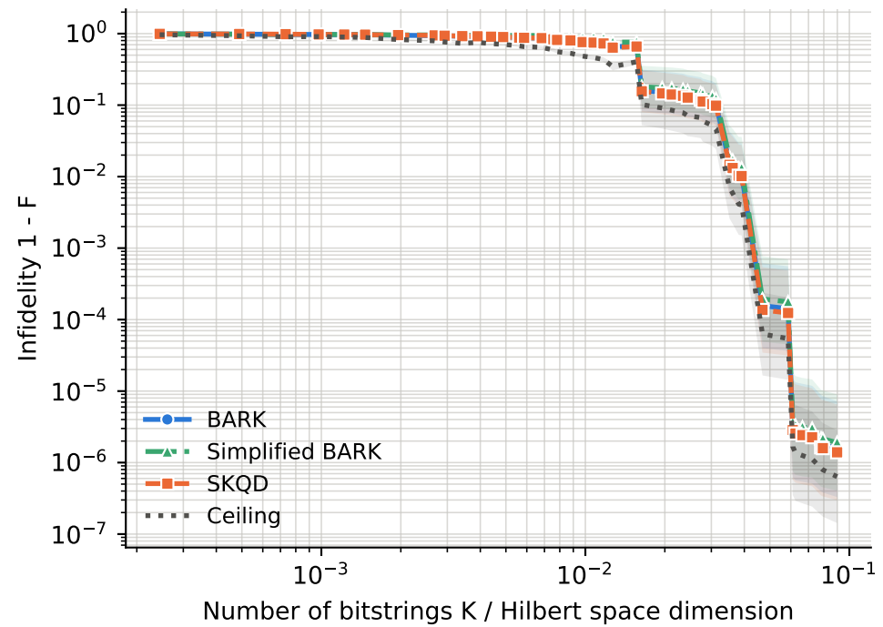
runs per point -- BARK: 22-108, Ceiling: 22-108, SKQD: 22-108, Simplified BARK: 22-108
