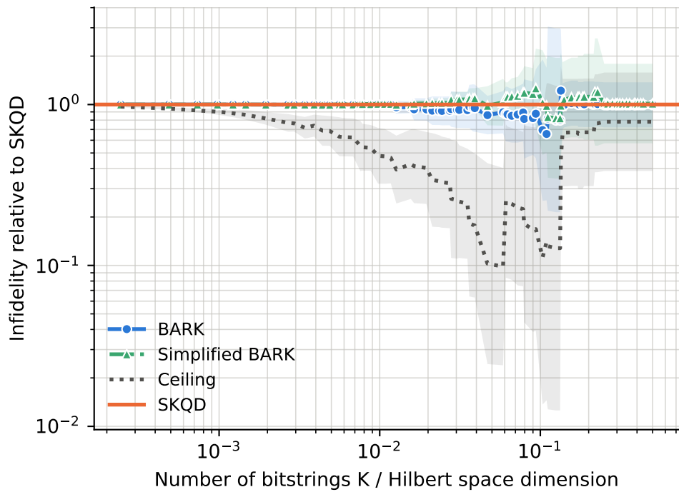
runs per point -- BARK: 13-21, Ceiling: 13-21, SKQD: 13-21, Simplified BARK: 13-21
