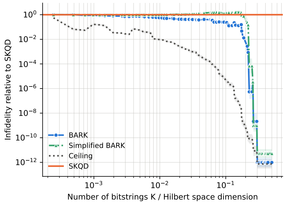
runs per point -- BARK: 33-115, Ceiling: 33-115, SKQD: 33-115, Simplified BARK: 33-115
