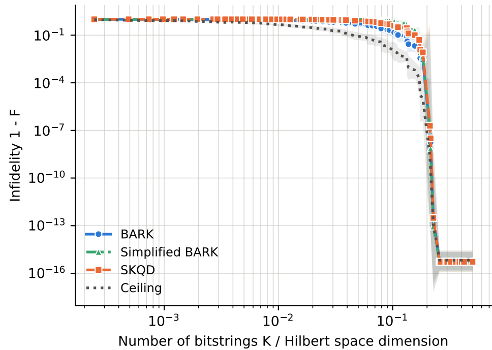
runs per point -- BARK: 19-47, Ceiling: 19-47, SKQD: 19-47, Simplified BARK: 19-47
