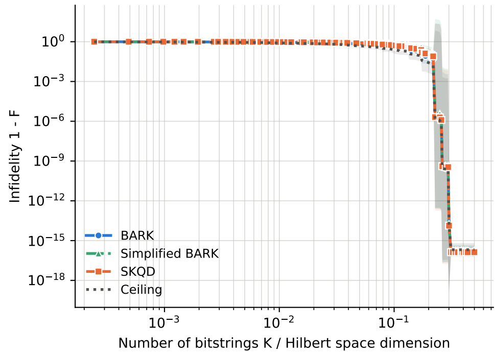
runs per point -- BARK: 9-29, Ceiling: 9-29, SKQD: 9-29, Simplified BARK: 9-29
