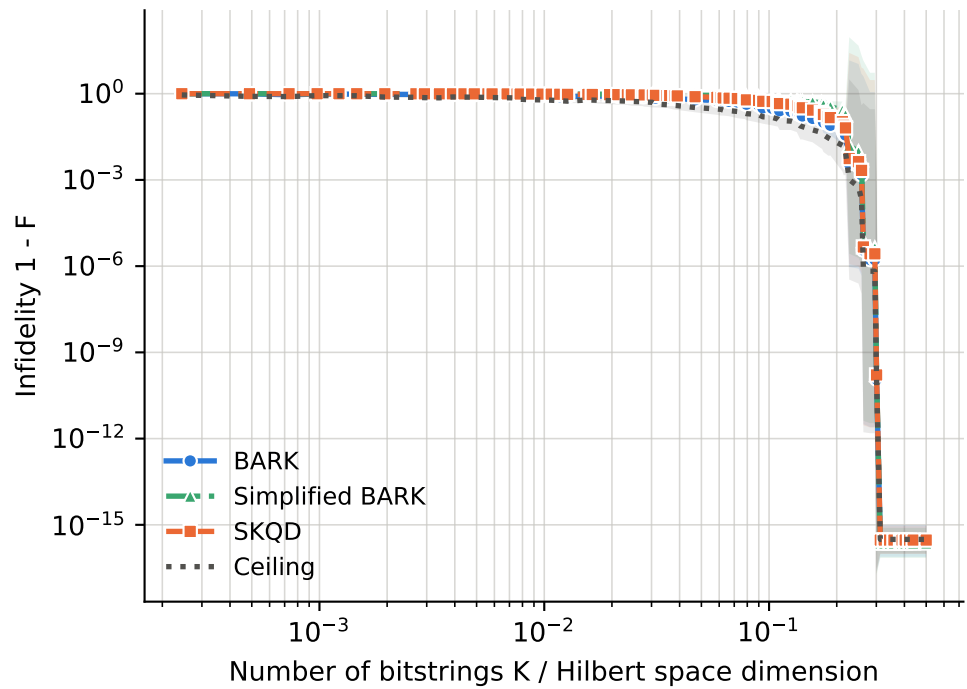
runs per point -- BARK: 4-51, Ceiling: 4-51, SKQD: 4-51, Simplified BARK: 4-51
