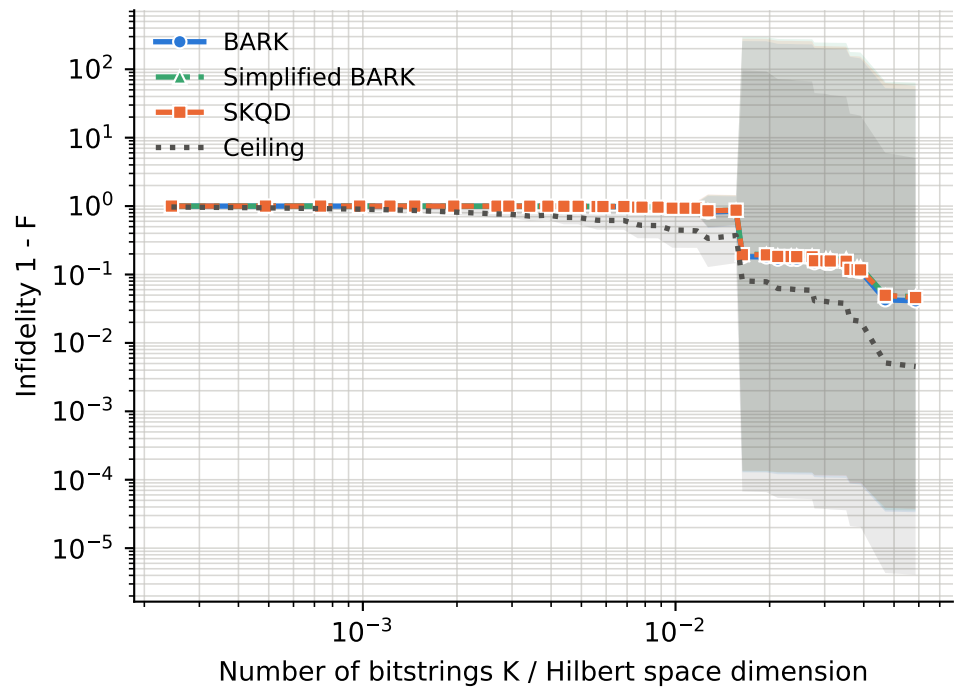
runs per point -- BARK: 13-21, Ceiling: 13-21, SKQD: 13-21, Simplified BARK: 13-21
