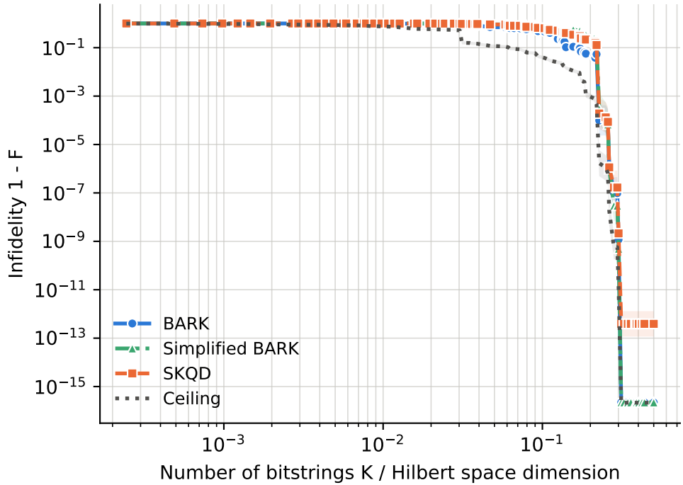
runs per point -- BARK: 16-83, Ceiling: 16-83, SKQD: 16-83, Simplified BARK: 16-83
