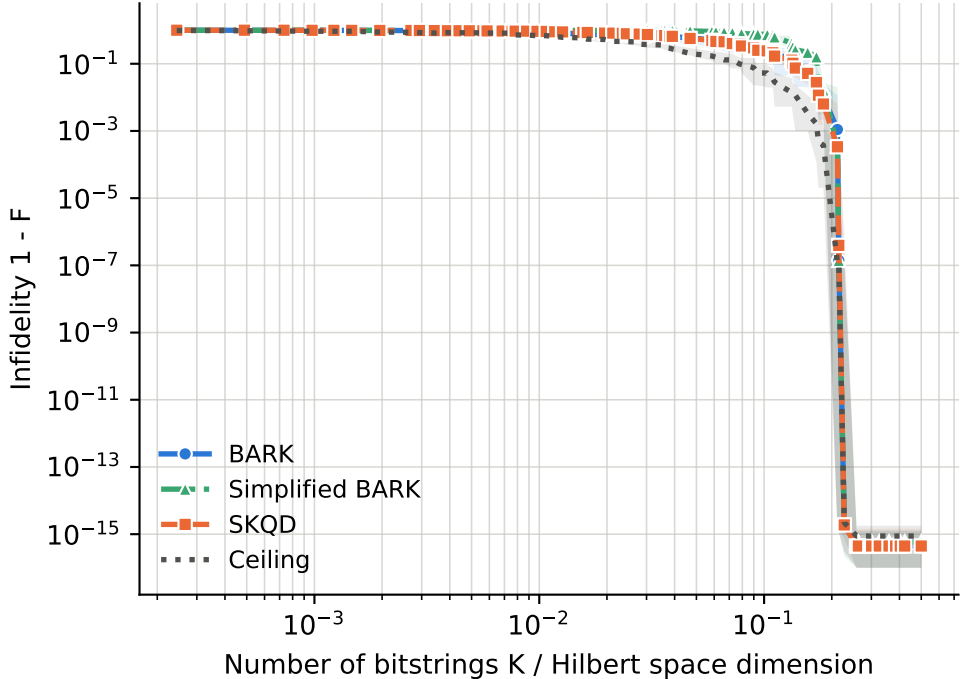
runs per point -- BARK: 11-44, Ceiling: 11-44, SKQD: 11-44, Simplified BARK: 11-44
