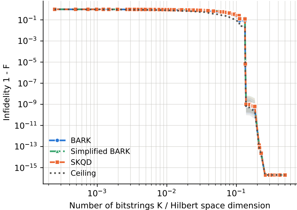
runs per point -- BARK: 31-96, Ceiling: 31-96, SKQD: 31-96, Simplified BARK: 31-96
