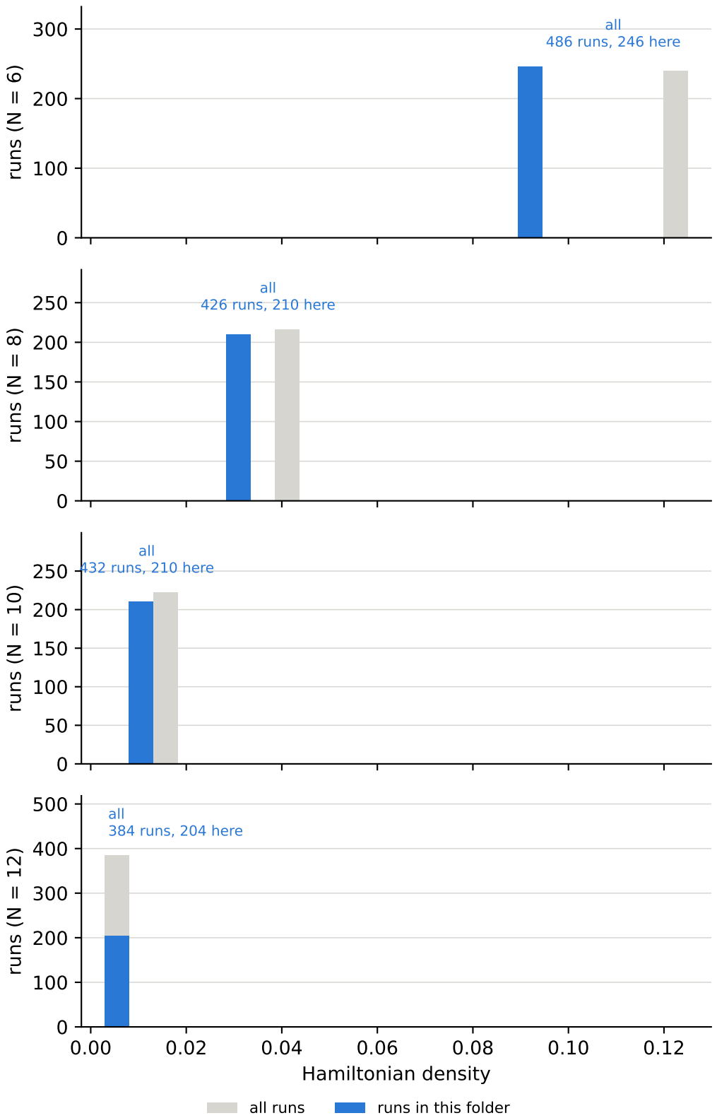
Hamiltonian density over all runs, and the cuts behind the bins lattice dimension = 1, Hamiltonian density = all
