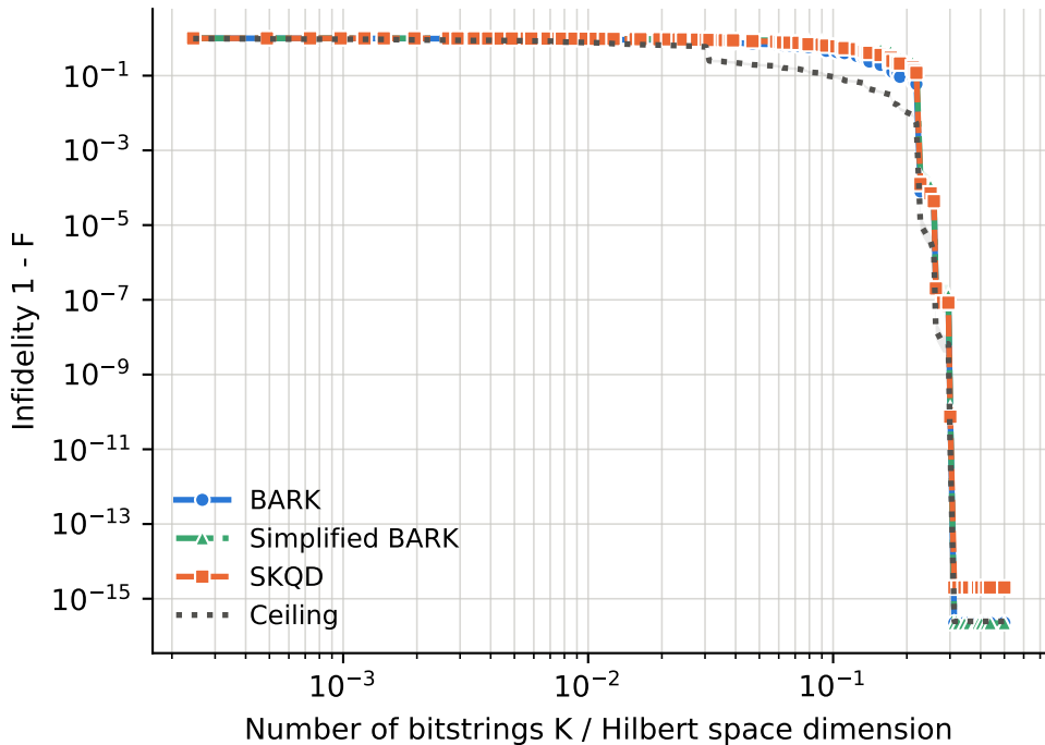
ground-state density = high (band: standard error)
