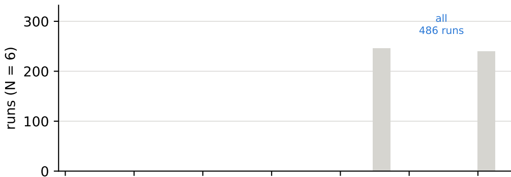
Hamiltonian density over all runs, and the cuts behind the bins Hamiltonian density = all
