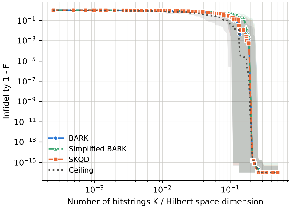
runs per point -- BARK: 128-571, Ceiling: 128-571, SKQD: 128-571, Simplified BARK: 128-571
