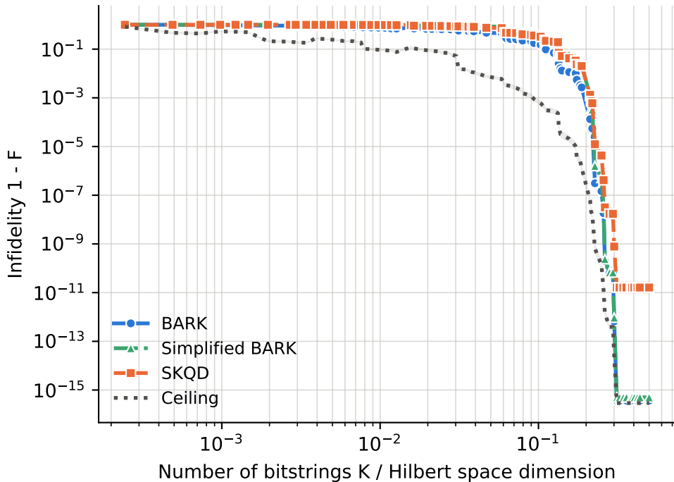
Hamiltonian density = all, initial overlap = low (band: standard error)
