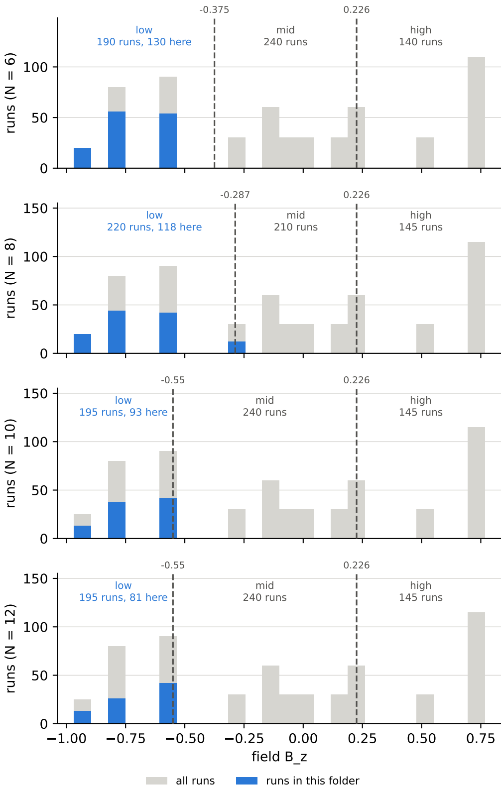
field B_z over all runs, and the cuts behind the bins field B_z = low, ground-state density = low
