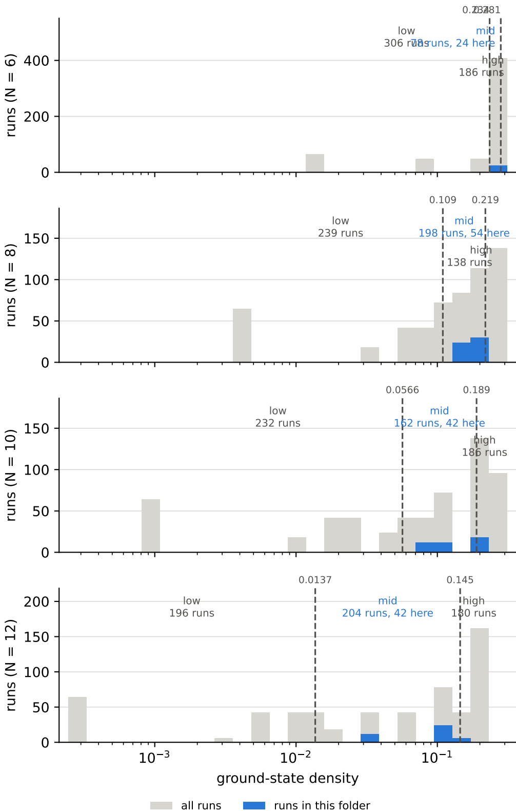
ground-state density over all runs, and the cuts behind the bins field B_z = mid, ground-state density = mid
