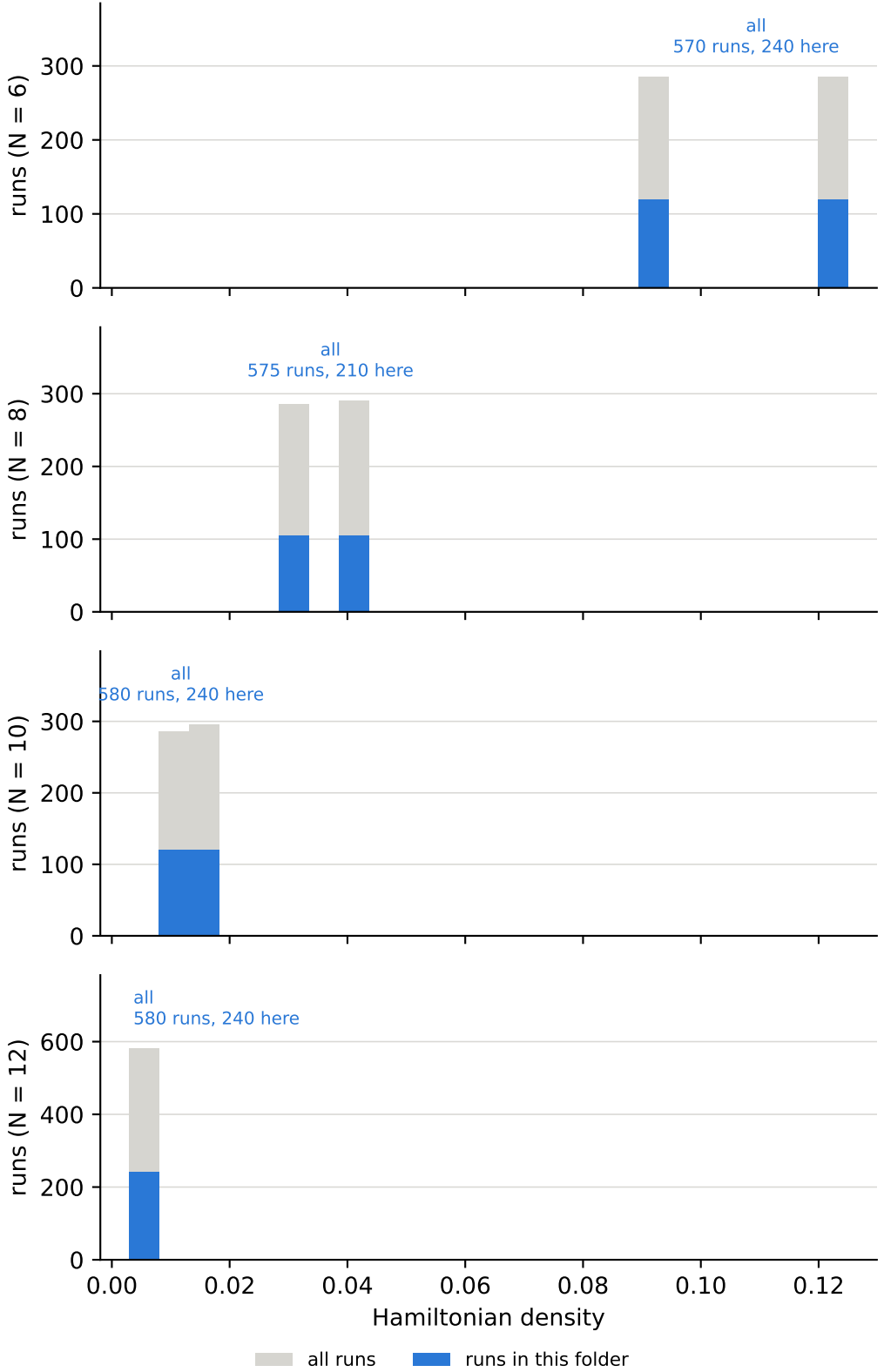
Hamiltonian density over all runs, and the cuts behind the bins field B_z = mid, Hamiltonian density = all
