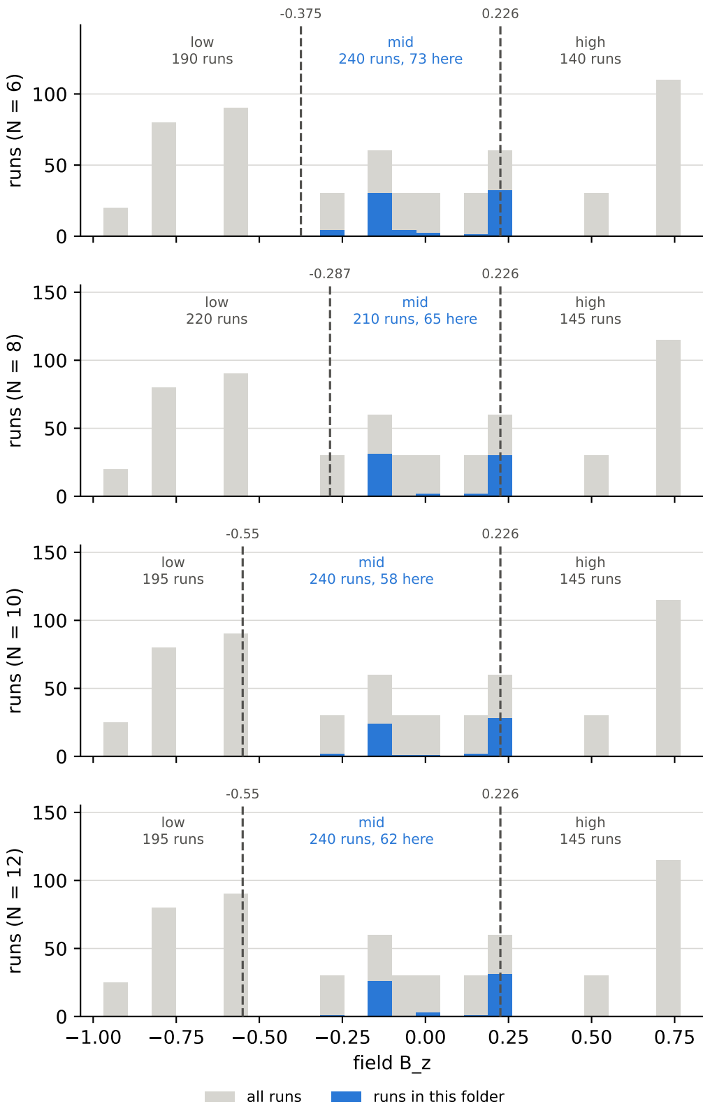
field B z over all runs, and the cuts behind the bins field B z = mid, initial overlap = low
