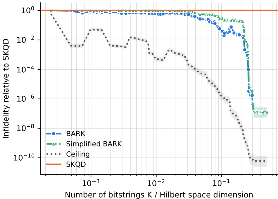
runs per point -- BARK: 92-356, Ceiling: 92-356, SKQD: 92-356, Simplified BARK: 92-356
