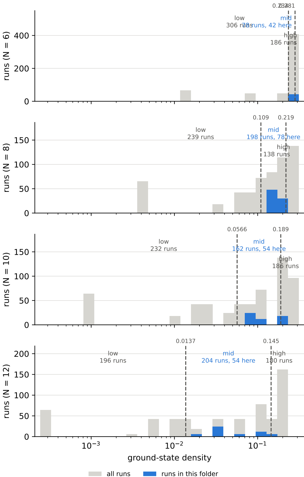
ground-state density over all runs, and the cuts behind the bins coupling J = mid, ground-state density = mid
