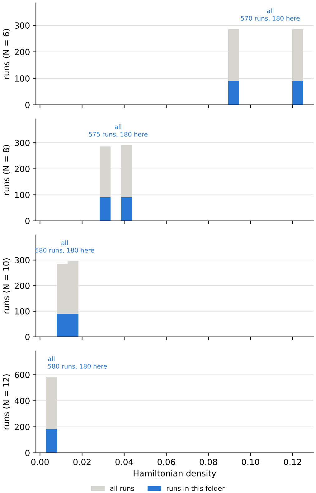
Hamiltonian density over all runs, and the cuts behind the bins coupling J = high, Hamiltonian density = all
