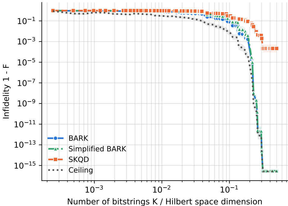
runs per point -- BARK: 51-193, Ceiling: 51-193, SKQD: 51-193, Simplified BARK: 51-193
