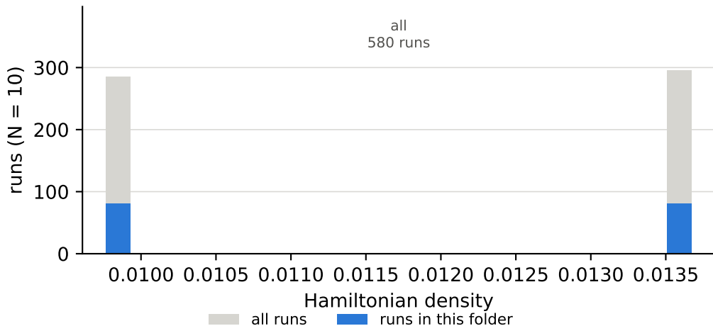
Hamiltonian density over all runs, and the cuts behind the bins N = 10 , anisotropy \delta = 0
