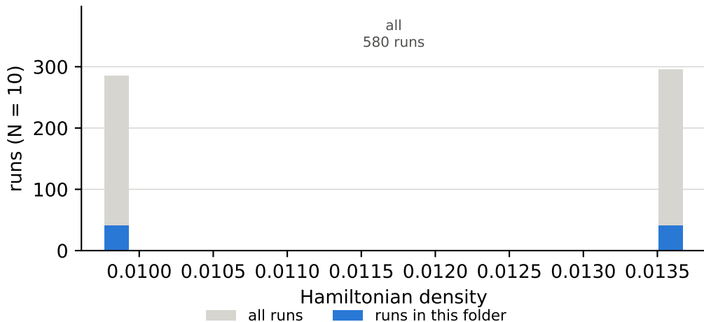
Hamiltonian density over all runs, and the cuts behind the bins N = 10 , anisotropy \delta = 1
