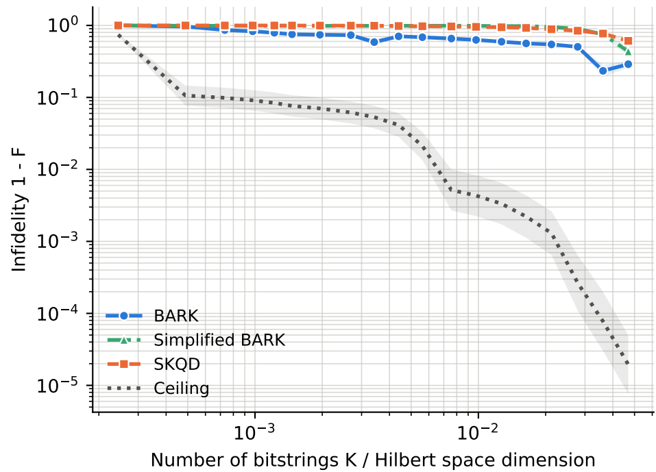
runs per point -- BARK: 90, Ceiling: 90, SKQD: 90, Simplified BARK: 90
