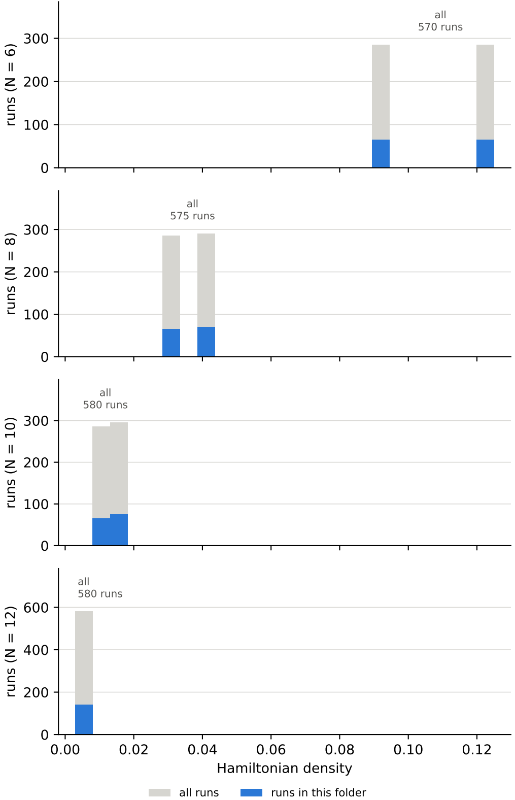
Hamiltonian density over all runs, and the cuts behind the bins anisotropy \Delta = 0.5
