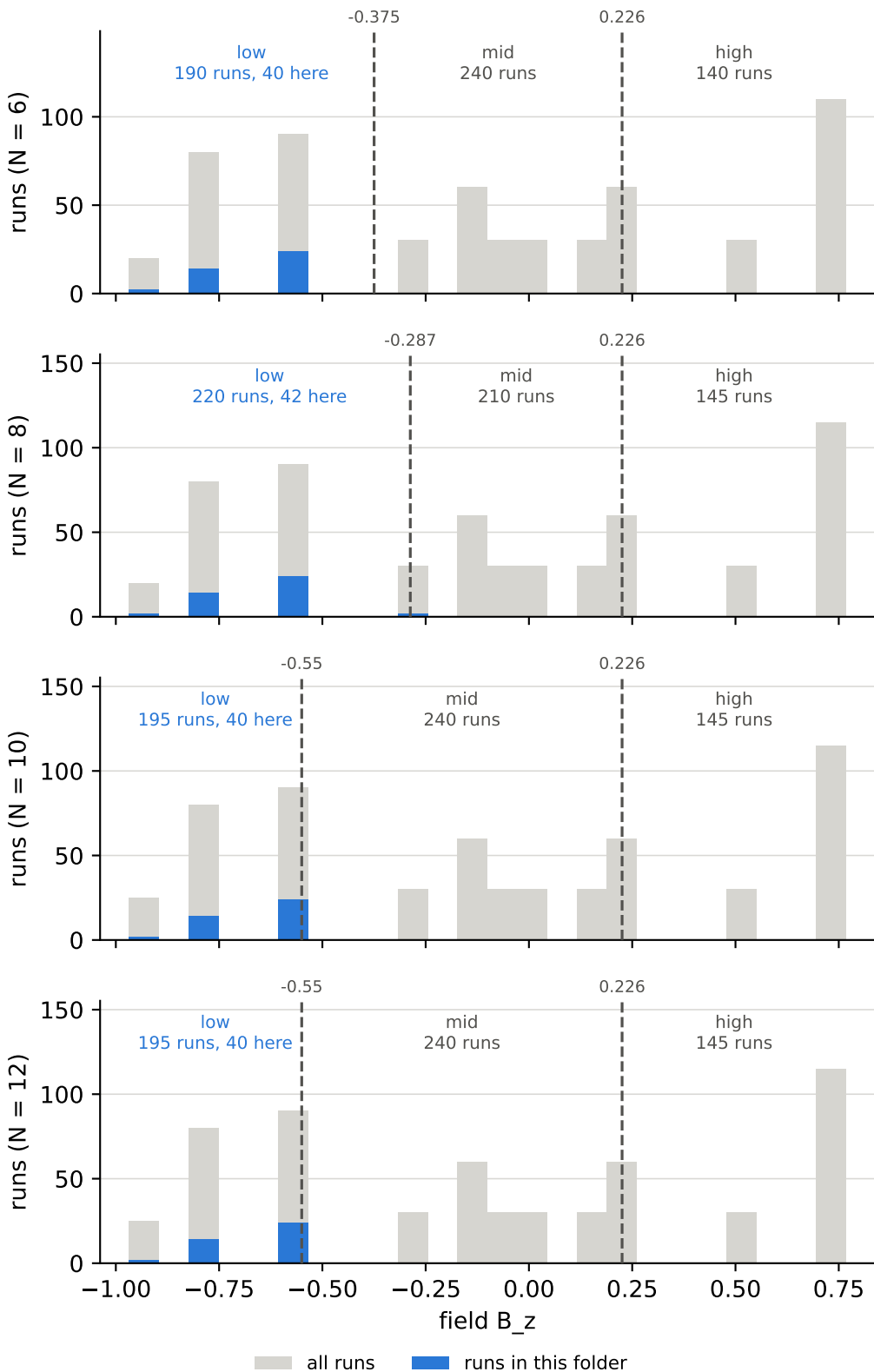
field B z over all runs, and the cuts behind the bins anisotropy delta = 10, field B z = low
