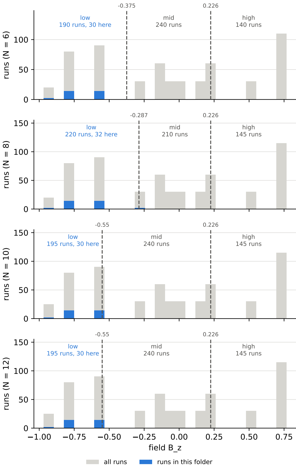
field B_z over all runs, and the cuts behind the bins anisotropy \delta = 1 , field B_z = low
