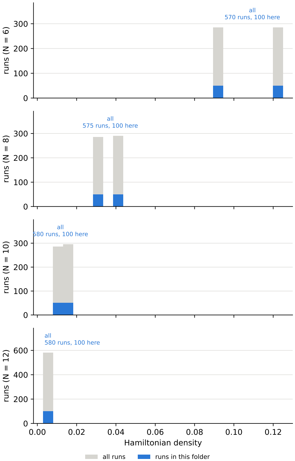
Hamiltonian density over all runs, and the cuts behind the bins anisotropy delta = 10, Hamiltonian density = all
